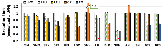
Fig. 10: Execution time with different eviction policies
