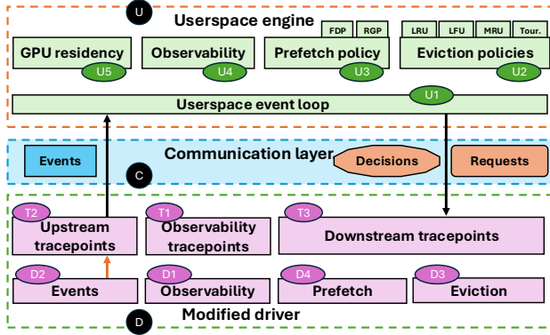
Fig. 6: Components of ObservUVM and their interactions
