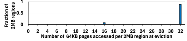
Fig. 5: Locality in 2MB regions upon eviction
