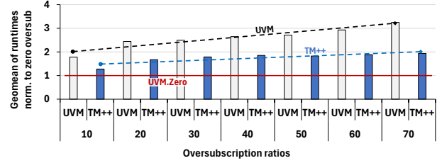
Fig. 15: ObservUVM with different oversubscription levels
