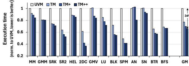
Fig. 9: Execution time with TM, TM+, and TM++
