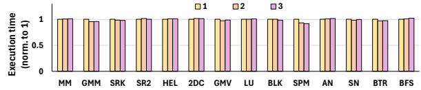
Fig. 17: Sensitivity to number of samples per region
